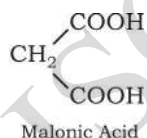
Malonic Acid
