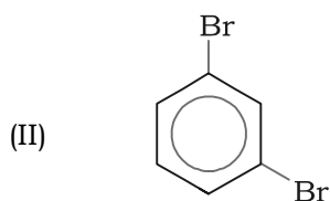
m-Dibromobenzene 1,3-Dibromobenzene
