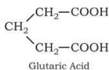
Glutaric Acid
