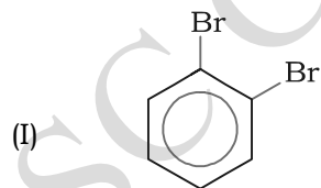
o-Dibromobenzene 1,2-Dibromobenzene
