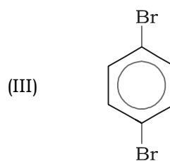
p-Dibromobenzene 1,4-Dibromobenzene
